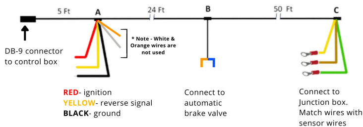
Schematic: 5 ft to A (cab), 24 ft to B (brake valve), 50 ft to C (junction box).
