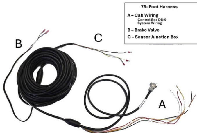
75-foot harness with three labeled branches: A – Cab Wiring, B – Brake Valve, C – Sensor Junction Box.
