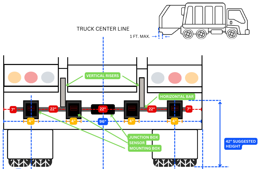
Mounting box placement (GS4000): four boxes across a 96" bumper, 22" between adjacent boxes, 7" from outer edges, at 42" height.
